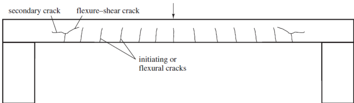
Figure: Flexure cracks and Flexure Shear or secondary Cracks
